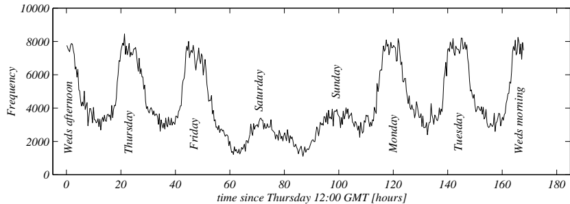
Figure 1: Histogram: Last-modified times (GMT), mod 24 \times 7 hours. Peaks in modification frequency are clearly visible during US working hours, and diminish on weekends. Any assumption of stationarity in page alteration probability will break down at this scale.
