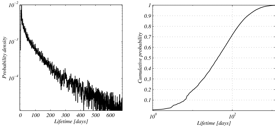
Figure 4: PDF and CDF of observed web page lifetimes. On the left, a rescaled histogram approximates the PDF of observed web page lifetimes, or differences in successive modification timestamps. On the right, we show the corresponding CDF. Note that these distributions are heavily influenced by the timespan of observation of single pages and also by the sample rate.
