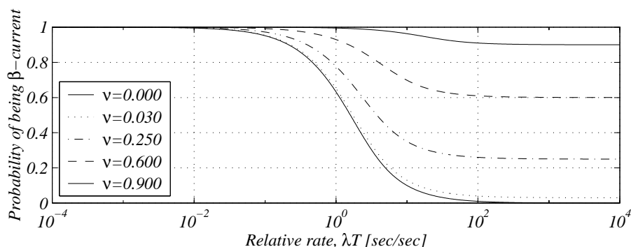
Figure 7: Probability of \beta -currency vs. relative rate for a single source . For a single Poisson source having change rate \lambda , re-indexed with period T , we plot the expected value of the probability \alpha as a function of relative rate z = \lambda T [dimensionless] and grace period percentage \nu = \beta/T during which unobserved changes are forgiven.
