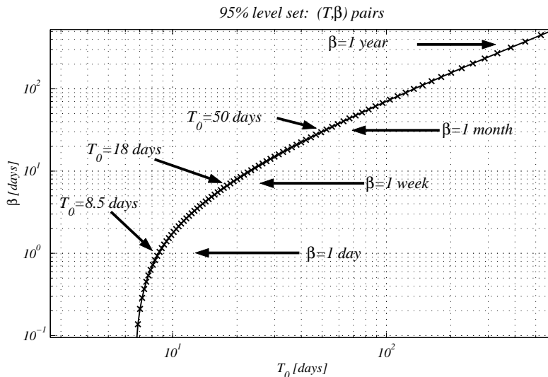
Figure 9: Relating \beta and T : \alpha=95\% level set. This is the level set of pairs (T, \beta) which for probability \alpha = 0.95 of being \beta -current. Regardless of the size of the collection, this data can be used to estimate how current an engine is when the indexing period T takes on a value (in days) along the horizontal axis. As T becomes large, the relative check rate is too slow, and \beta approaches 0.95T .
