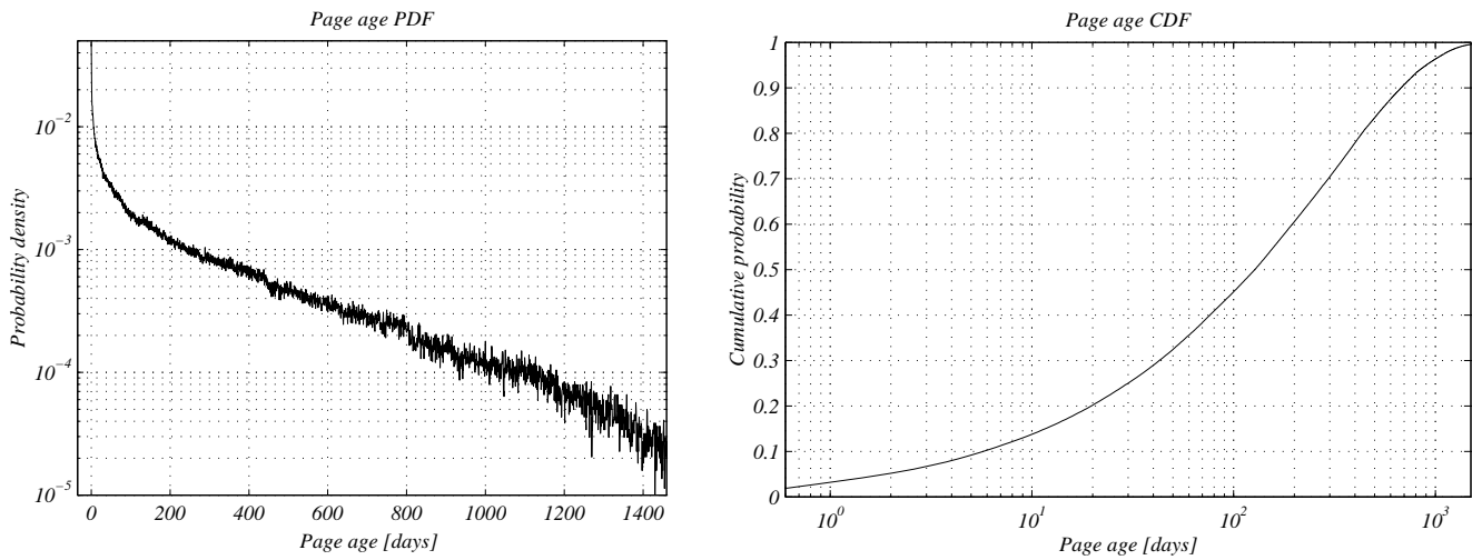
Figure 3: Distribution of web page ages. Here we show estimates of the probability density function (PDF) and cumulative distribution function (CDF) of web page age. On the left, we estimate the PDF using a rescaled histogram of web page ages, using one age observation per page. On the right, the corresponding CDF is formed by integrating the estimate of the PDF.
