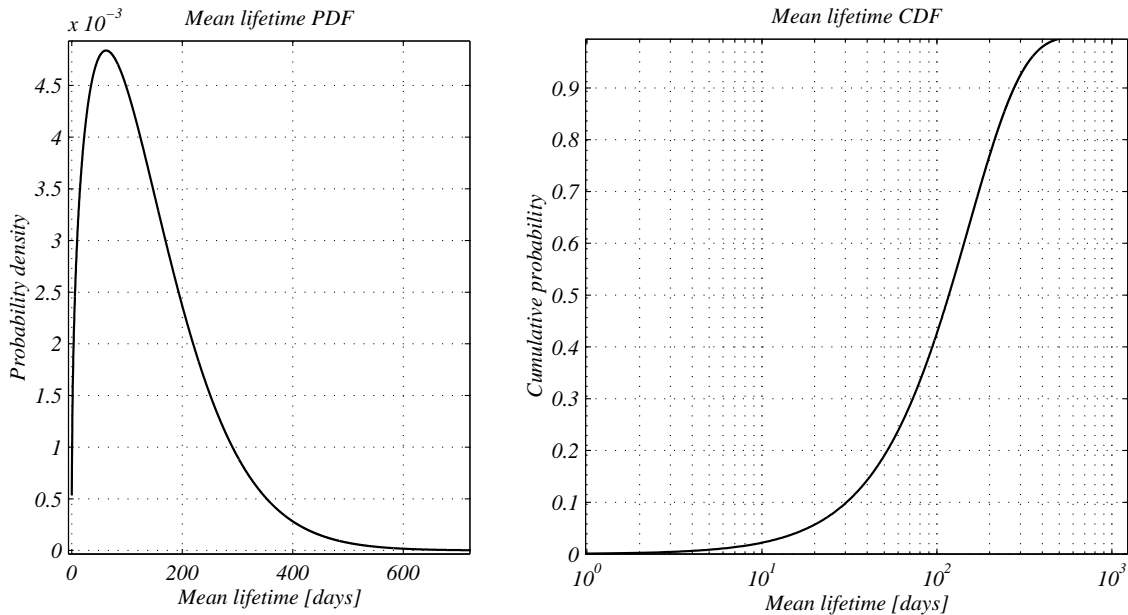
Figure 5: Estimated PDF and CDF of mean web page lifetime \bar{t} . Parameter estimation implies these distributions of mean lifetimes \bar{t} for the documents observed by the Informant. Note that these mean values (or inverse change rates) are to be distinguished from the distribution of observed lifetimes shown in Figure 4. The average is around 138 days, the maximum of the PDF occurs at 62 days, and the median is 117 days.
