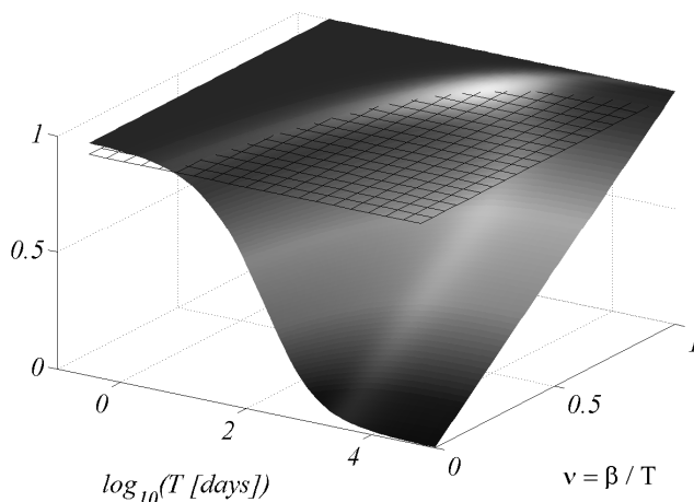
Figure 8: Probability \alpha for an entire collection as a function of \nu = \beta/T and T : The probability surface \alpha for a collection of sources with a rate distribution diagrammed in Figure 5. The plane at \alpha = 0.95 intersects the surface in a level set, which is plotted in Figure 9 (with \beta values used instead of percentages \nu ).
