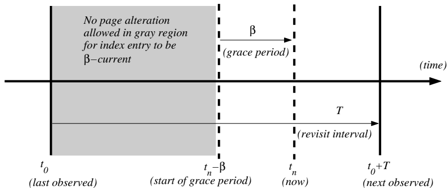
Figure 6: Definition of “ \beta -current” . This diagram shows what is meant when we say that an index entry is current with respect to a grace period, \beta . In order to be \beta -current, no modification can go unobserved up to \beta time units before the present.
