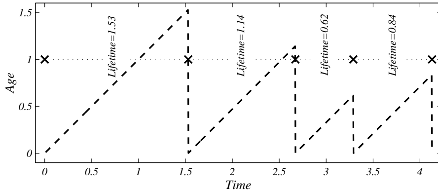
Figure 2: Lifetimes vs. ages. A single lifetime is represented by the time separating changes, which are denoted by \times 's in the graph. For each lifetime, the age (shown as a dashed line) increases linearly from 0 to the lifetime, then resets to 0 as the next lifetime begins.
